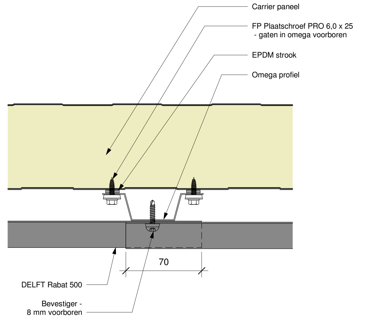
Detail - Overlap
